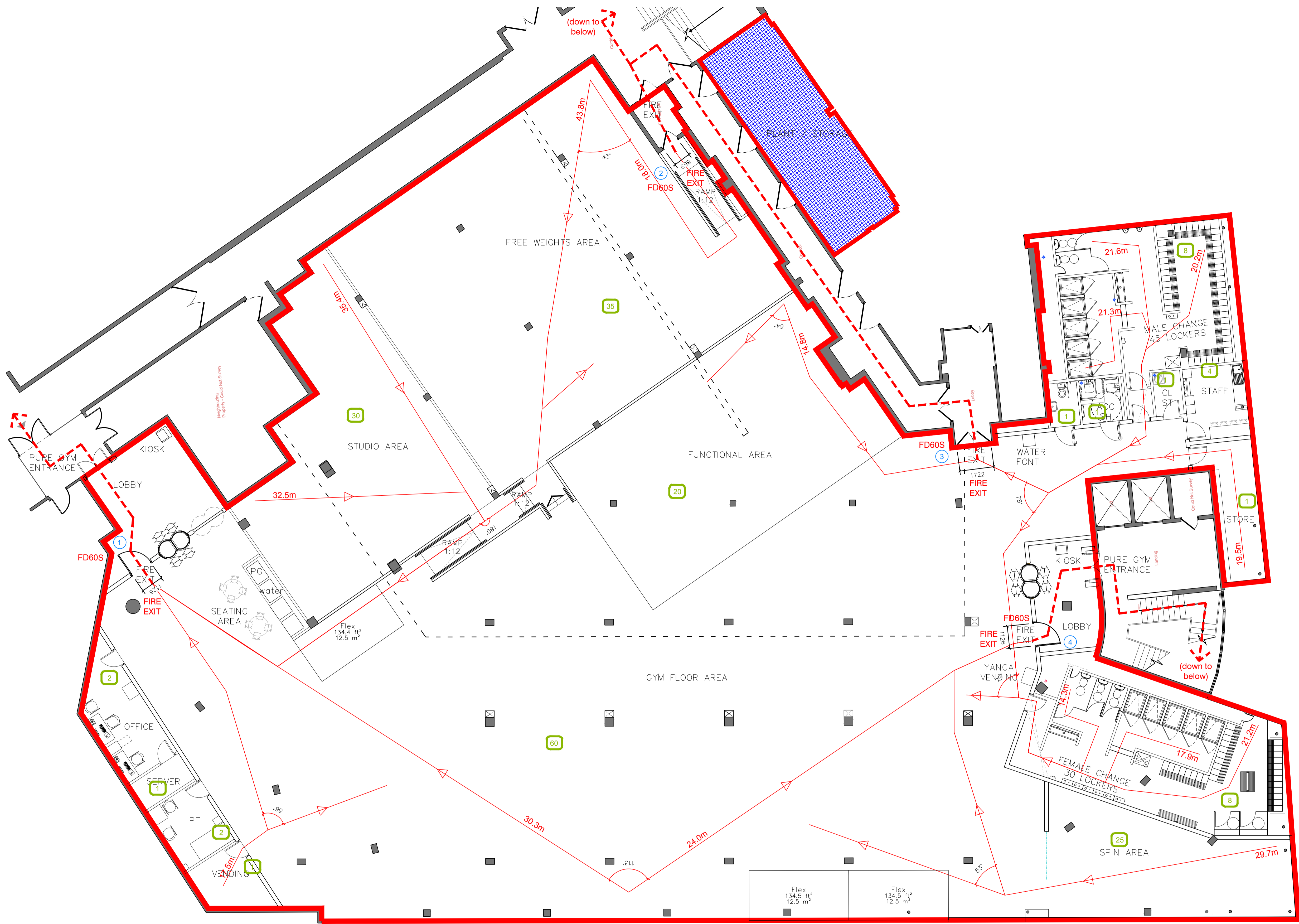
Ground Floor Fire Evacuation Plan 1:100
